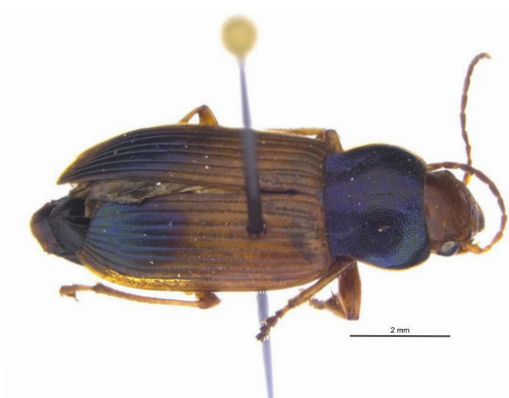
Figure 2: Dorsal view of Diachromus germanus collected from the area of cut trees in the grazed coastal secondary grassland (Sammet et al. 2023) 2 . Photo by Olavi Kurina.
